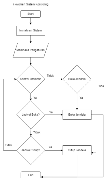
Gambar 6. Alur Flowchart Sistem Kontroling
