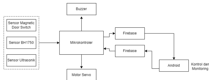
Gambar 3. Blok Diagram
